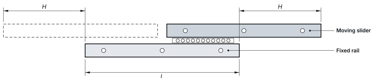
Fig. 9 VT-P two-way: with the stop screw removed the slider extends by H to either side (dashed)
