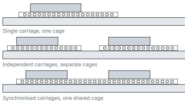
Fig. 4 VT-L carriage configurations
