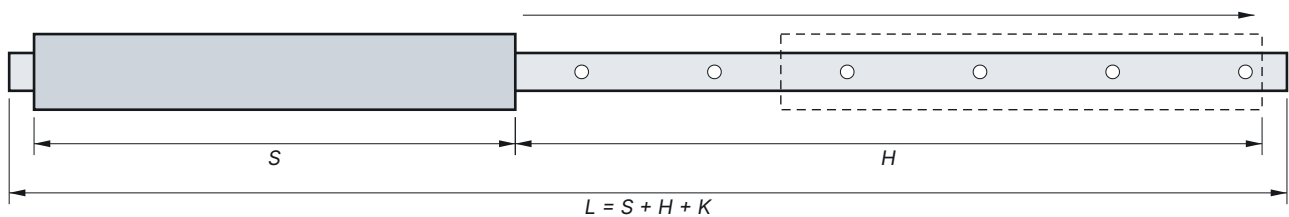
Fig. 3 VT-L — rail length L = carriage length S + stroke H + end allowance K (example VT-L35.290.450.770)
