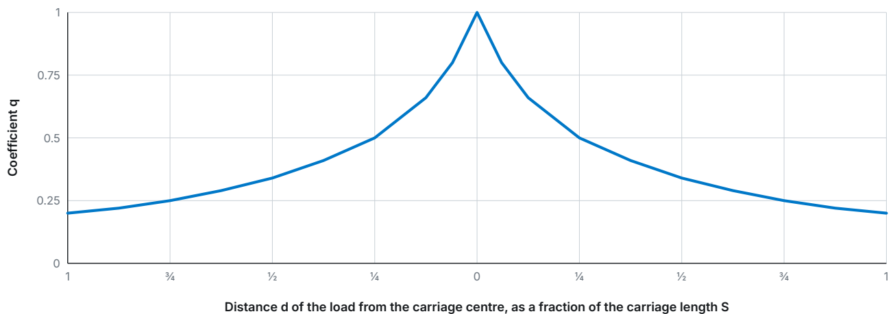
Fig. 33 Position coefficient q : 1 at the carriage centre, falling symmetrically towards each end
