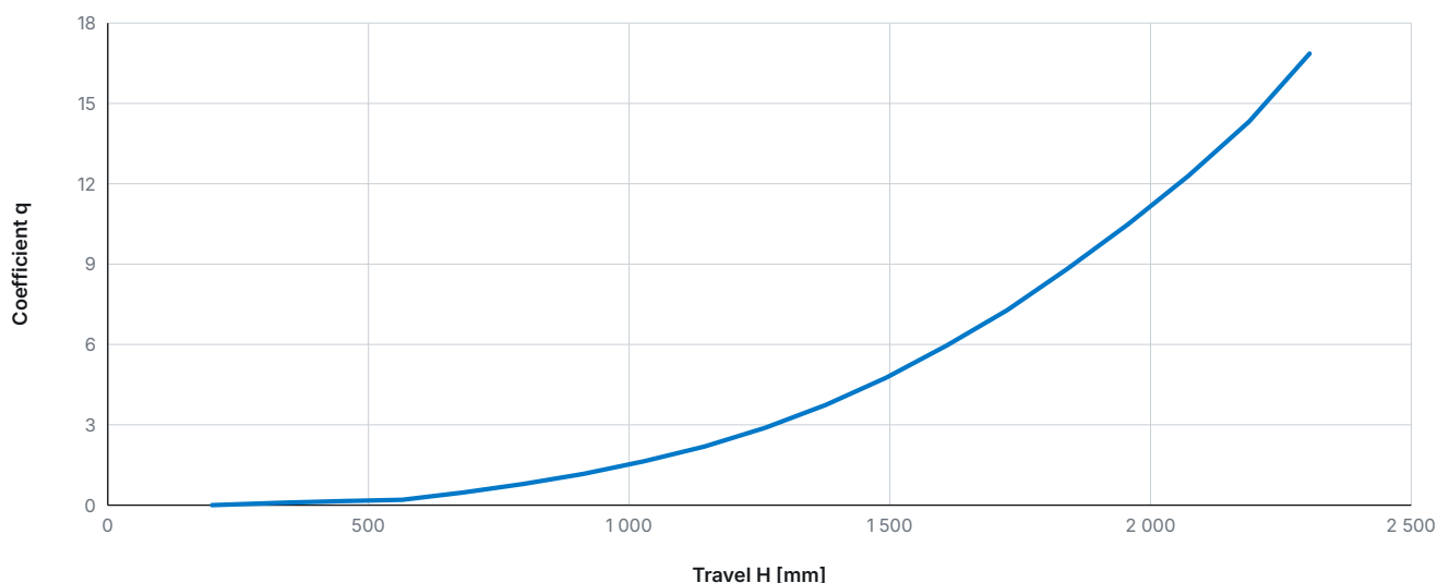
Fig. 26 Travel coefficient q as a function of the travel H — VT-X, VT-O and VT-H
