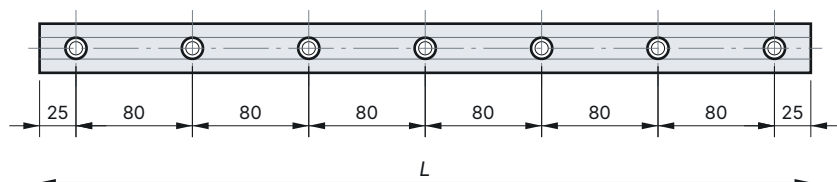
Fig. 11 Rail in plan view, example L = 530 mm: first hole 25 mm from each end, then 80 mm pitch
