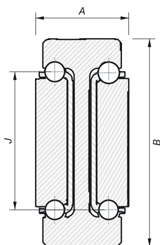
Fig. 22 Cross-section VT-H
