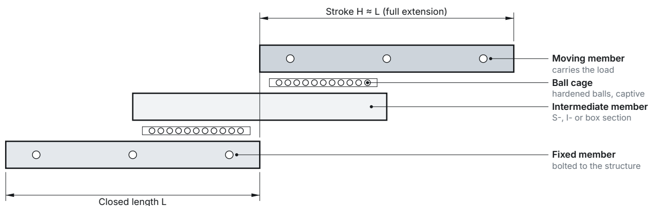
Fig. 1 Full-extension telescopic slide, fully extended (members drawn apart for clarity)
