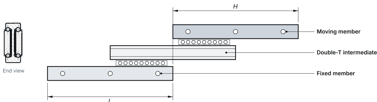
Fig. 21 VT-H extended: stroke H \approx closed length L ; intermediate member with double-T section
