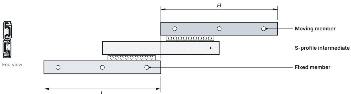
Fig. 12 VT-S1 extended: stroke H \approx rail length L (slightly more, see the size tables); VT-S2 extends to both sides
