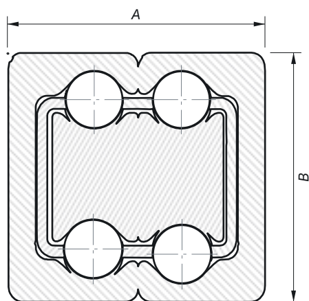
Fig. 19 Cross-section VT-O
