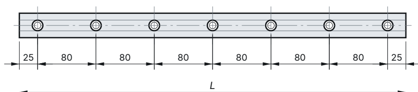
Fig. 20 Rail in plan view, example L = 530 mm: first hole 25 mm from each end, then 80 mm pitch
