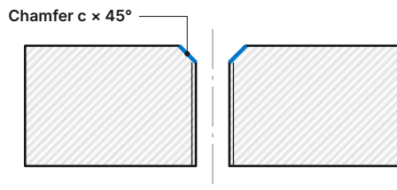
Fig. 29 Chamfer at the threaded fastening holes
