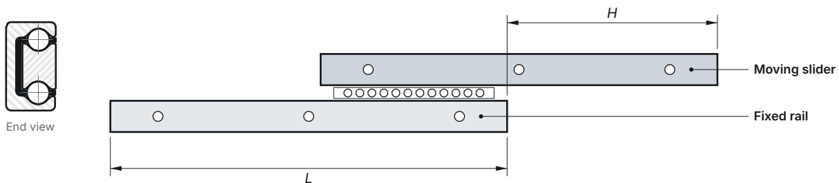
Fig. 8 VT-P extended: the slider travels H \approx 50\text{--}60\% of the closed length L ; there is no intermediate member
