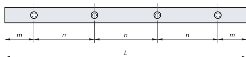
Fig. 23 VT-H rail in plan view: end distance m and pitch n per length, see the size tables
