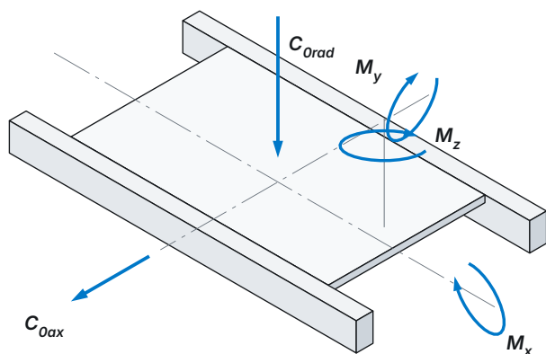
Fig. 2 Load and moment directions on an extended slide pair
