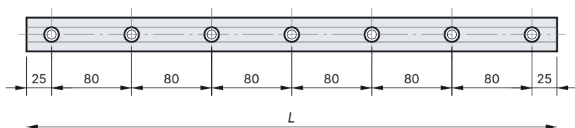
Fig. 17 Rail in plan view, example L = 530 mm: first hole 25 mm from each end, then 80 mm pitch
