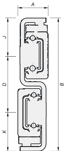
Fig. 13 Cross-section VT-S
