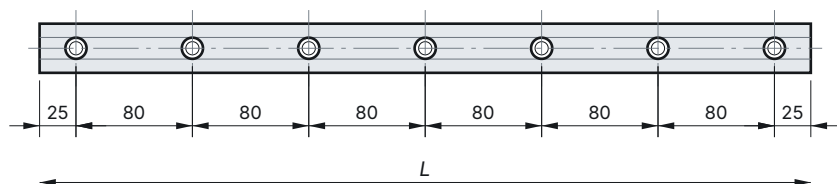
Fig. 6 Rail in plan view, example L = 530 mm: first hole 25 mm from each end, then 80 mm pitch
