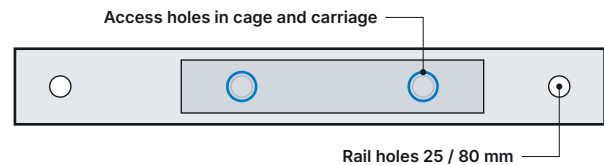
Fig. 32 Access holes in cage and carriage line up with the rail holes
