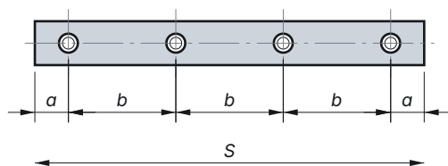
Fig. 7 Carriage in plan view, example S = 290 mm: hole offset a and pitch b for every carriage length in the size tables
