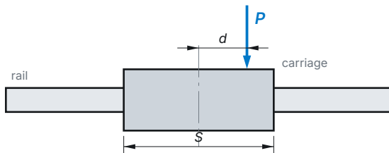
Fig. 31 Off-centre load P on the carriage
