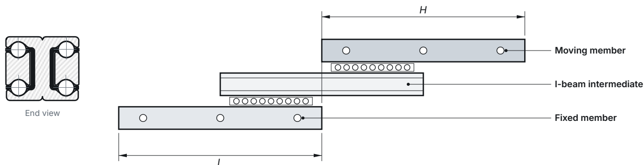
Fig. 15 VT-X extended: stroke H = closed length L (one-way); two-way with the end-stop screws removed
