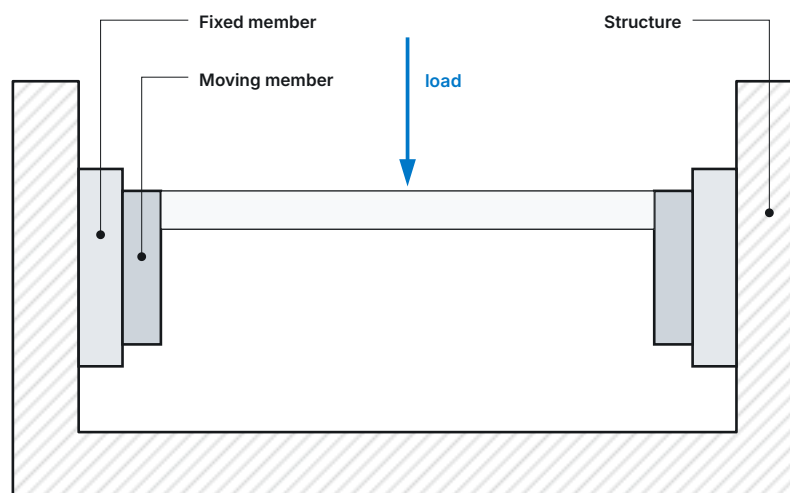
Fig. 30 Slide pair in a supporting structure: fixed members on the structure, load on the moving members
