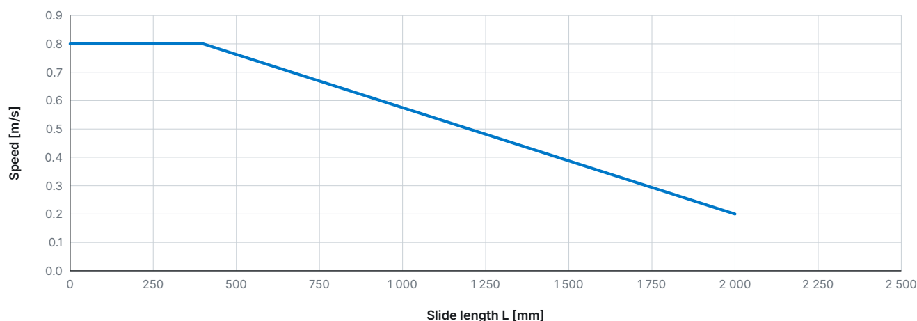
Fig. 28 Maximum operating speed as a function of the slide length
