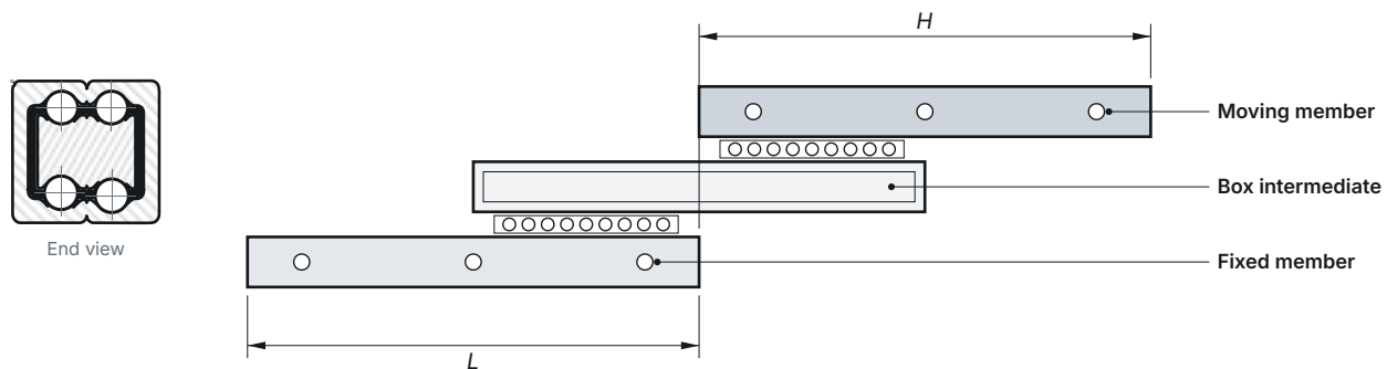
Fig. 18 VT-O extended: stroke H = closed length L ; two guide rails with the box intermediate between them
