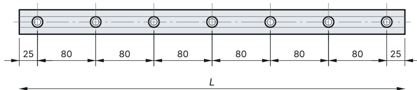
Fig. 14 Rail in plan view, example L = 530 mm: first hole 25 mm from each end, then 80 mm pitch
