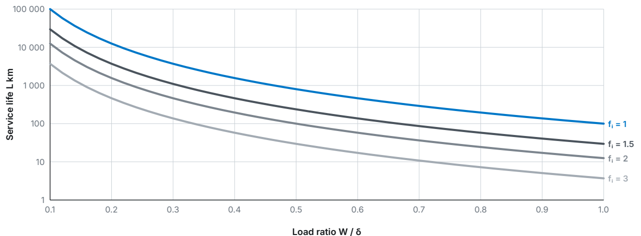
Fig. 27 Calculated service life from formula (4) for application coefficients f_i = 1 \dots 3
