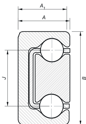
Fig. 5 Cross-section VT-L — rail and carriage
