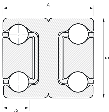
Fig. 16 Cross-section VT-X
